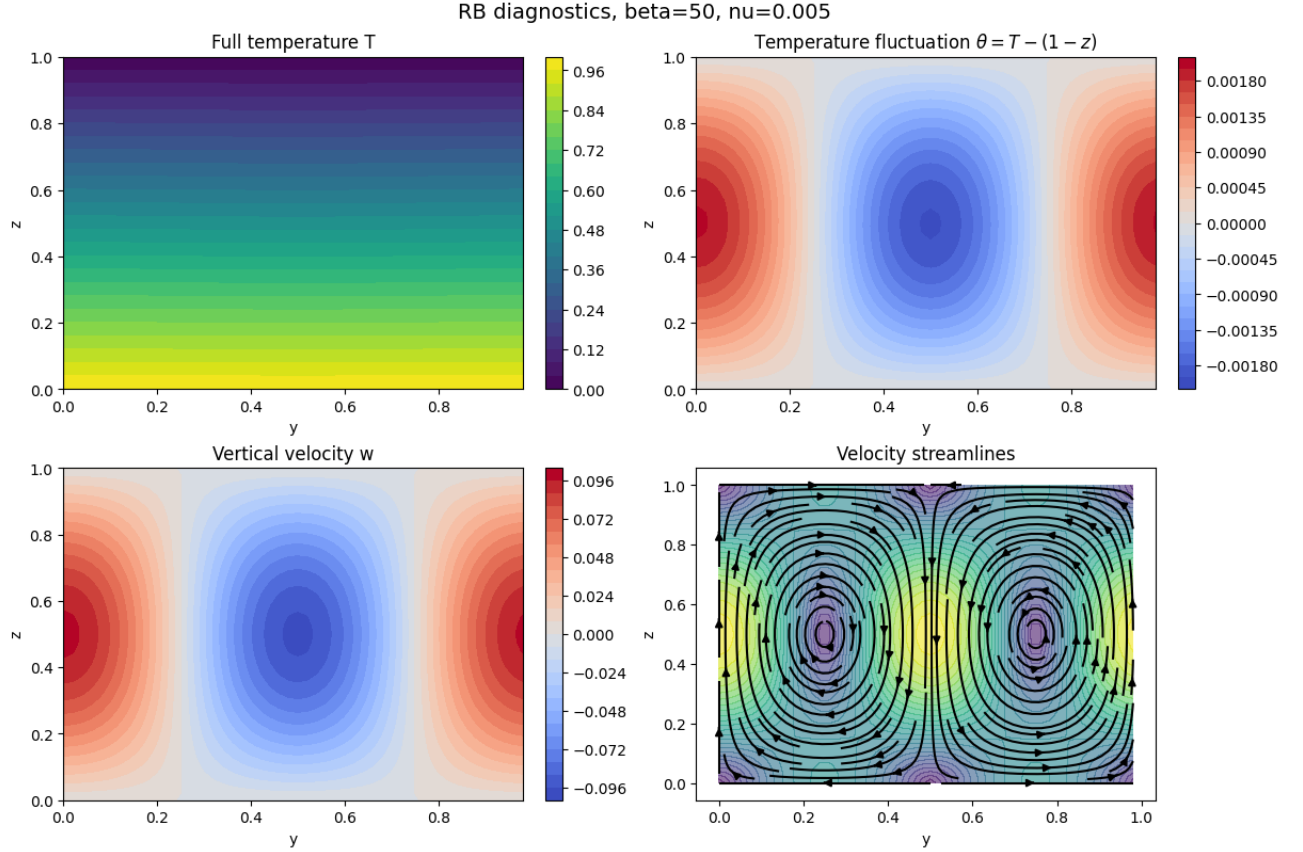
Figure 3.5: Results of the numerical solution for \beta = 50 , \nu = 0.005 . Results for a paramterisation causing Rayleigh-Bénard convection cells induced by thermal forcing (for thermal forcing see plot at the upper left).
