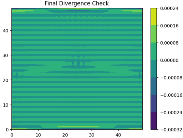
Figure 3.4: Divergence error at machine precision accuracy using FFT solver.
