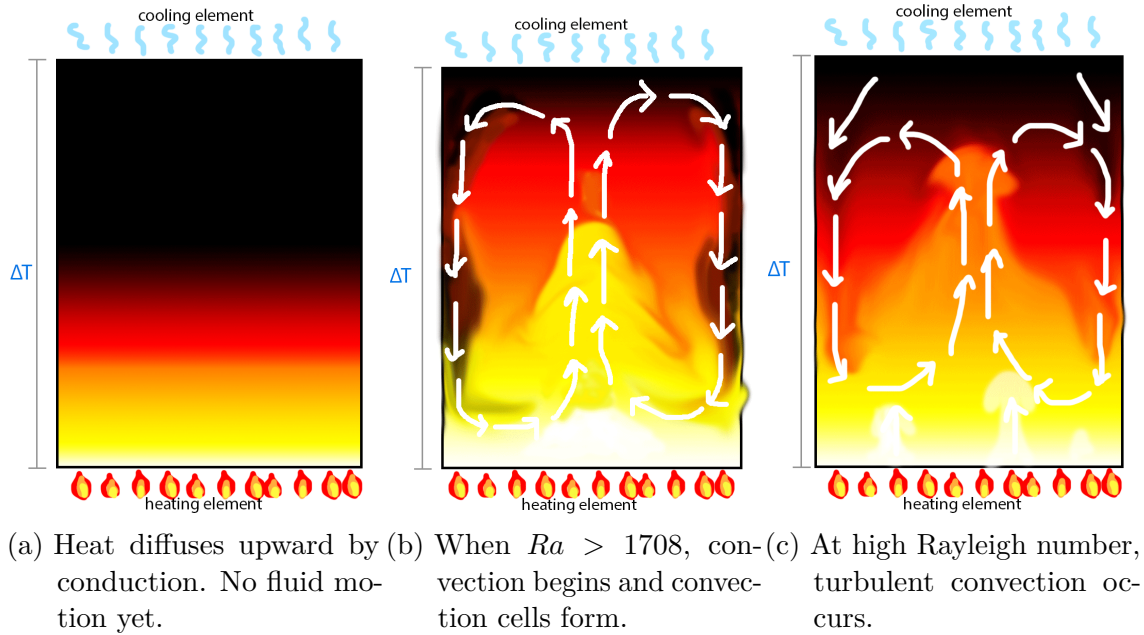
Figure 1.1: Rayleigh-Bénard Convection (Chang, n.d.)
